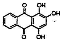
PURPURIN
